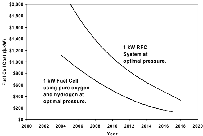
Figure 1. Extrapolated and projected fuel cells and RFC system costs. kW rating is for electrolysis.
