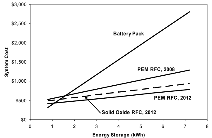
Figure 2. Projected costs of energy storage options based on eight hours between charging and constant power use between charging.
